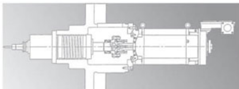
Motor Direct Driving Spindle for HMC-500/500H/630/630H
